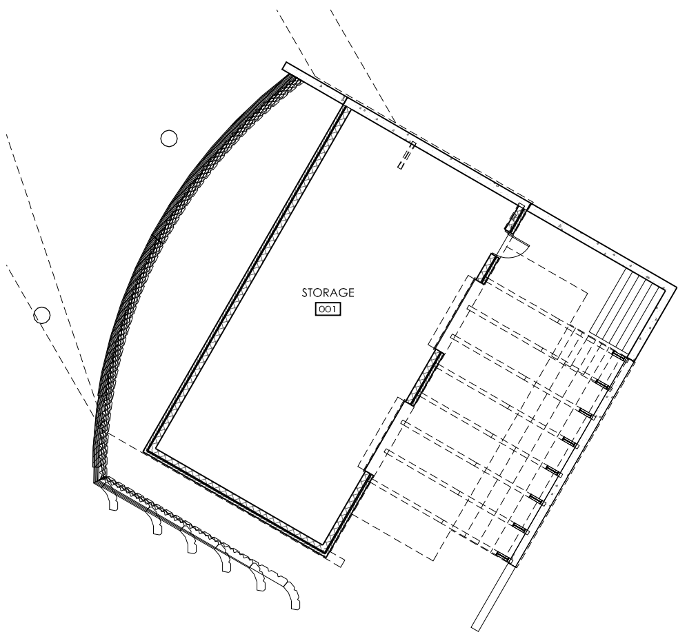
02 LOWER LEVEL FLOOR PLAN 1/8" = 1'-0"
